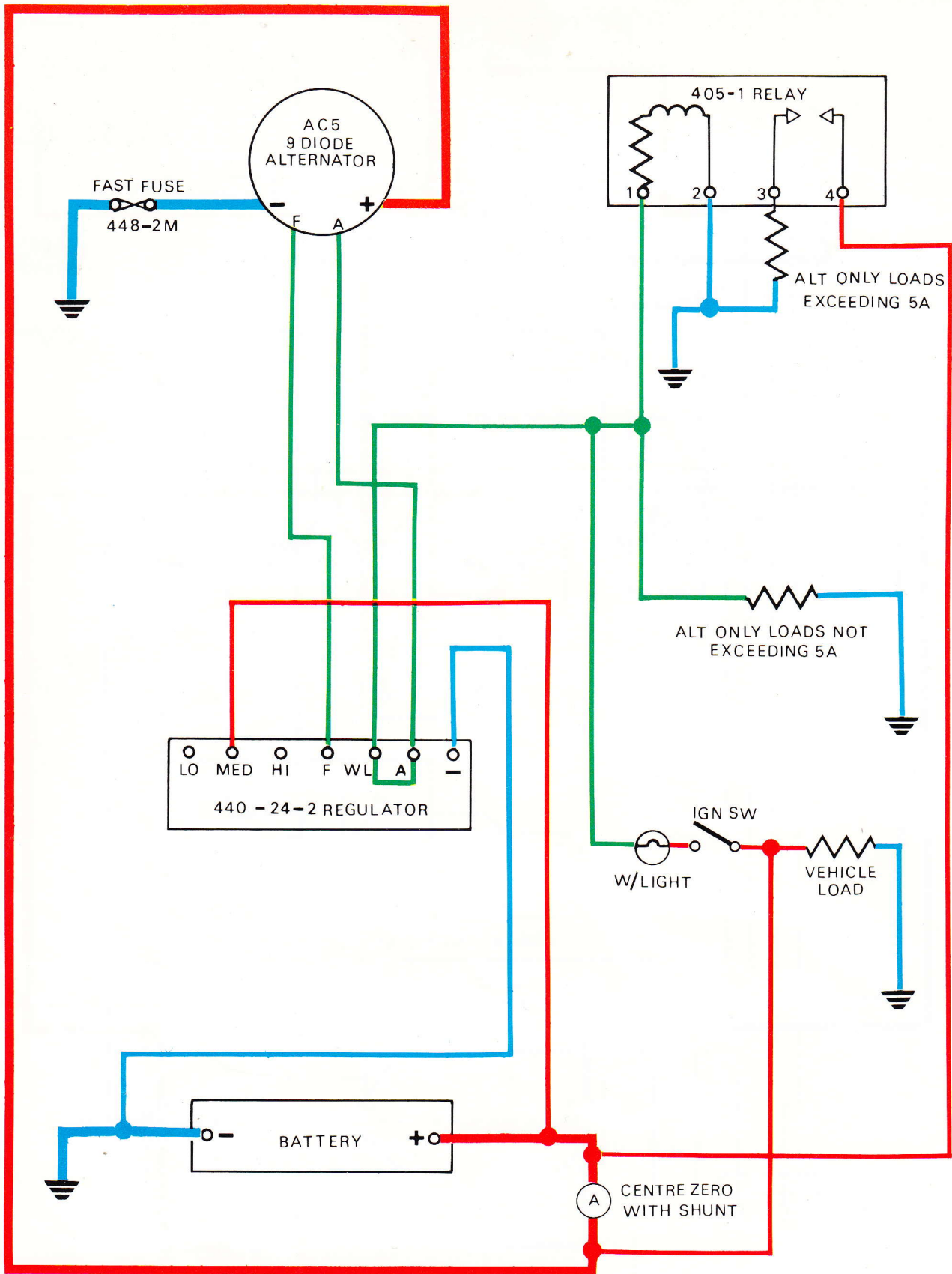
Fig 22 AC5 negative earth system
